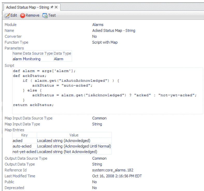
Figure 35. Script with Map Function example
