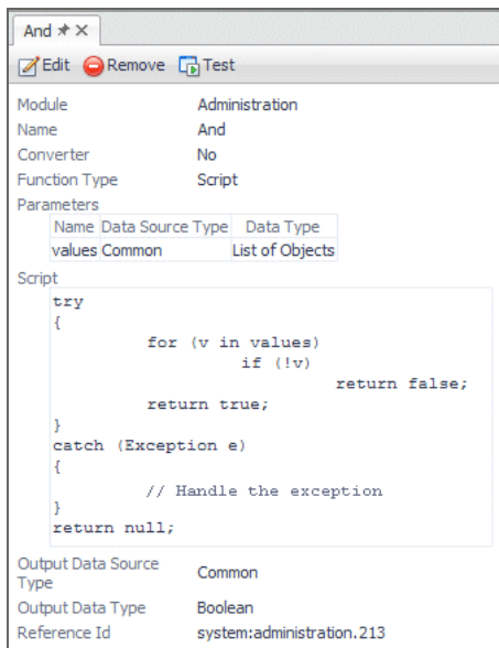
Figure 34. Script function example
