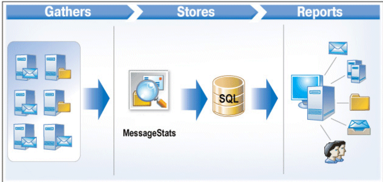
Figure 1. MessageStats workflow.
