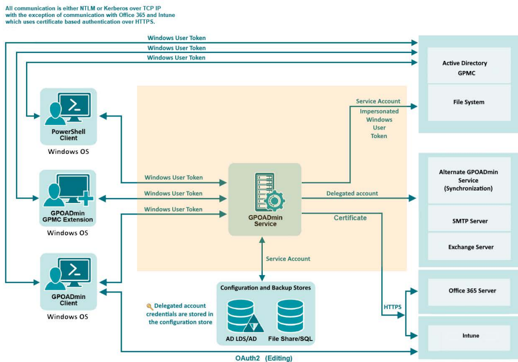
Figure 2. Architecture and Communication Overview
