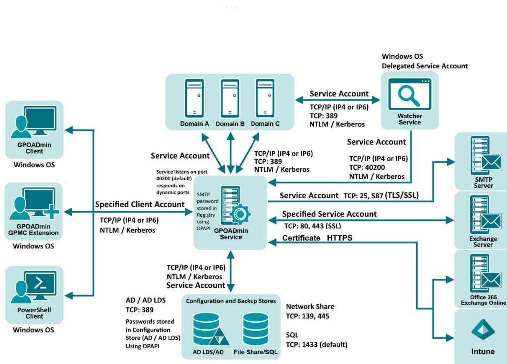
Figure 1. Communication Protocols Overview
