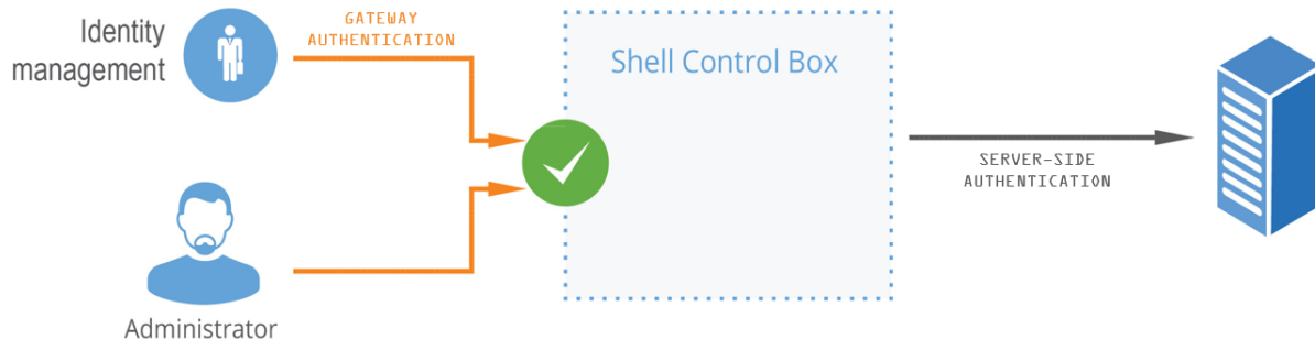
Figure 8: Gateway authentication
