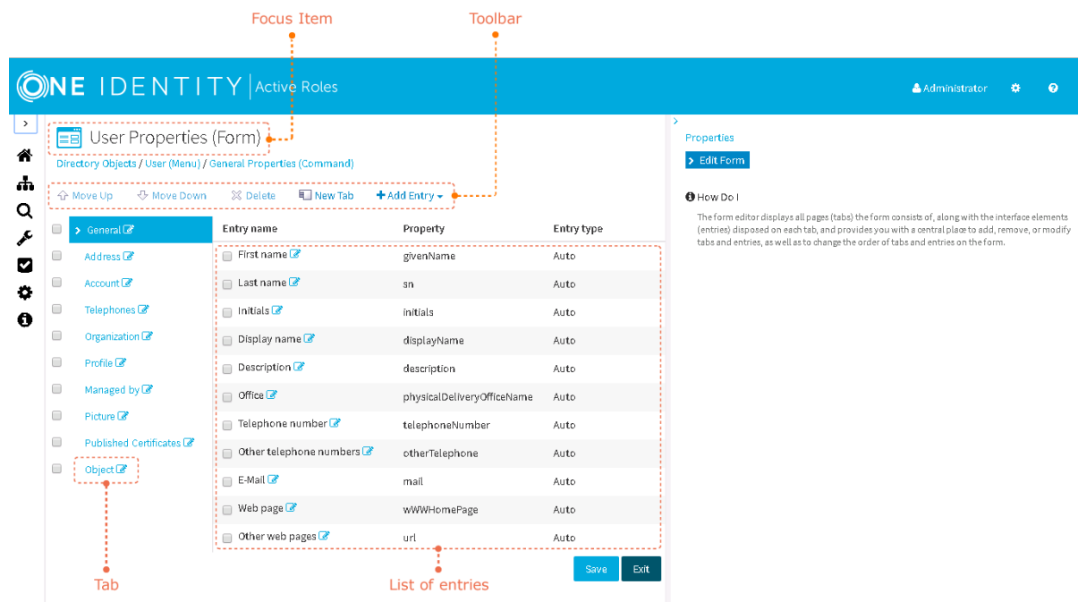
Figure 2: Form Editor
