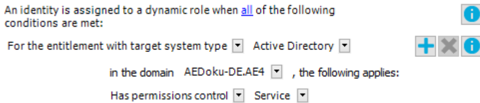
Figure 17: Filter designer
