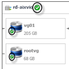
Figure 41. Health indicator
