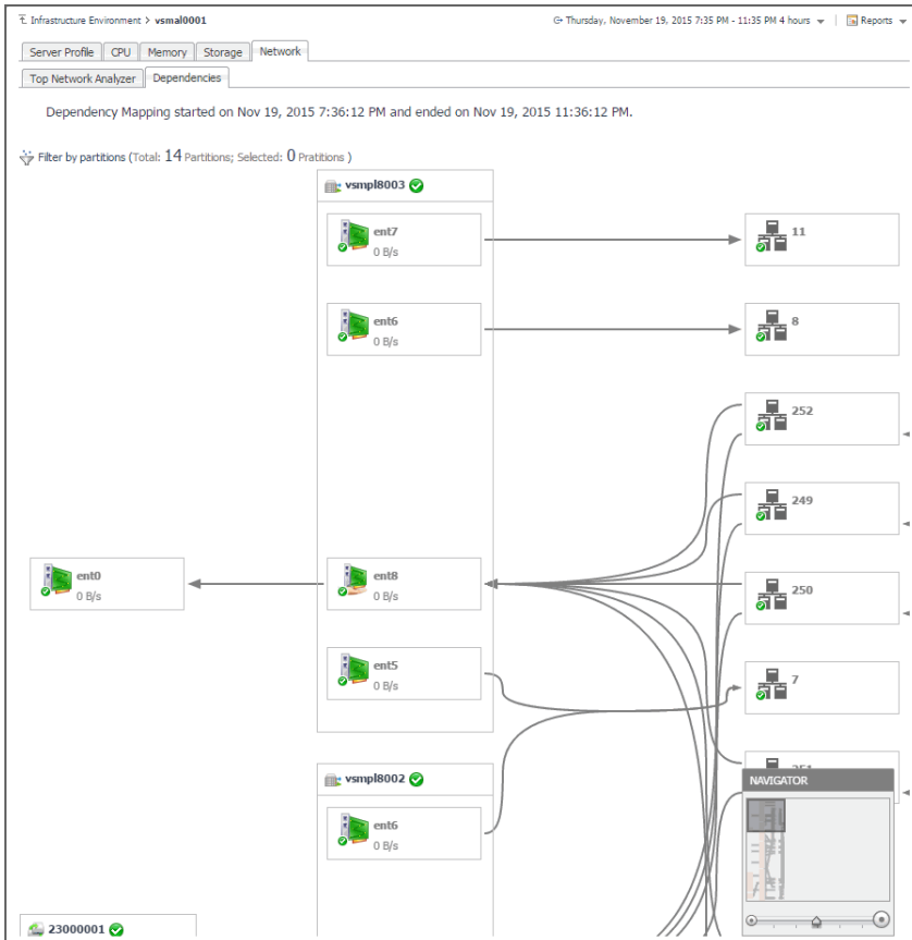
Figure 39. Dependency map
