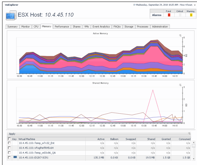
Figure 66. Memory tab
