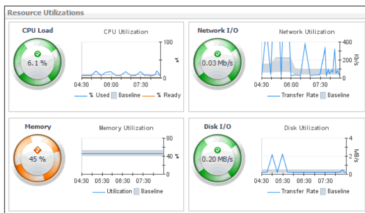
Figure 27. Resource Utilization views
