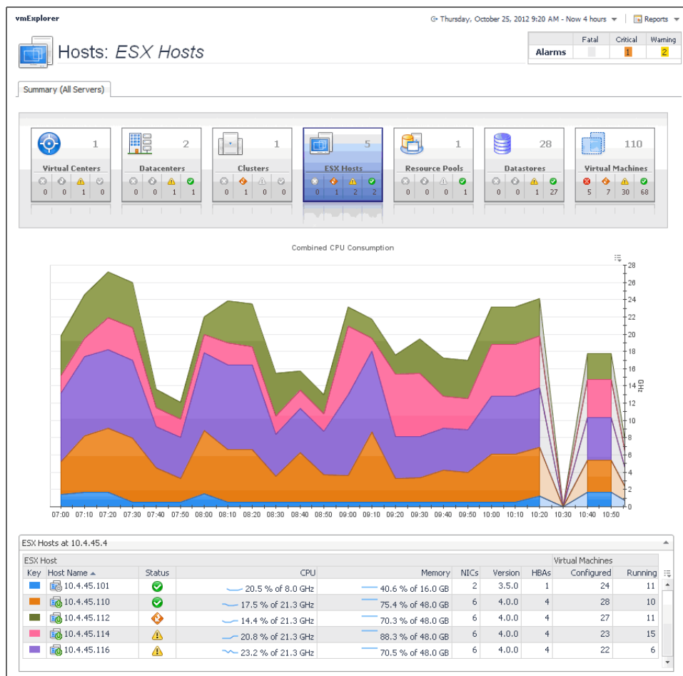
Figure 69. Summary (All Servers) tab
