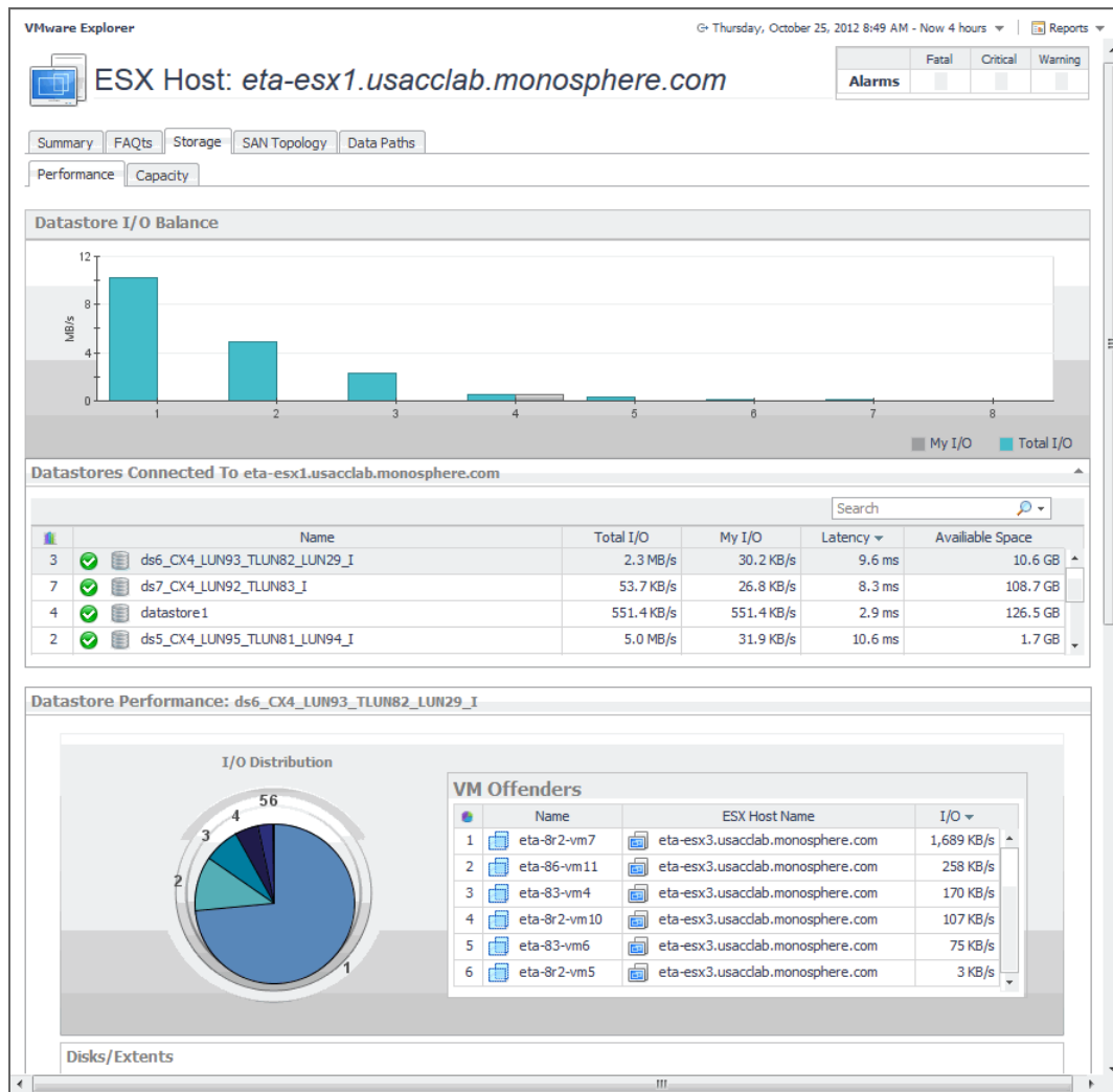
Figure 63. Storage tab (ESX Host)
