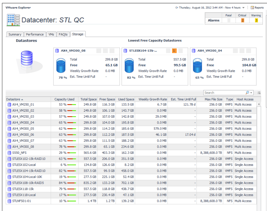
Figure 62. Storage tab (Datacenter)
