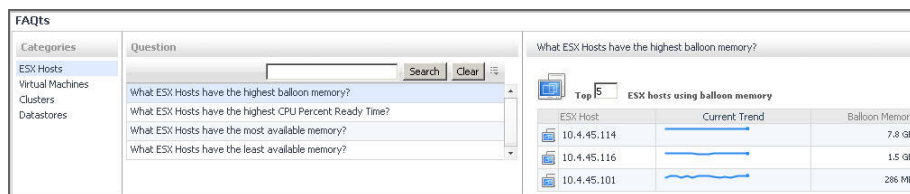
Figure 59. FAQs tab
