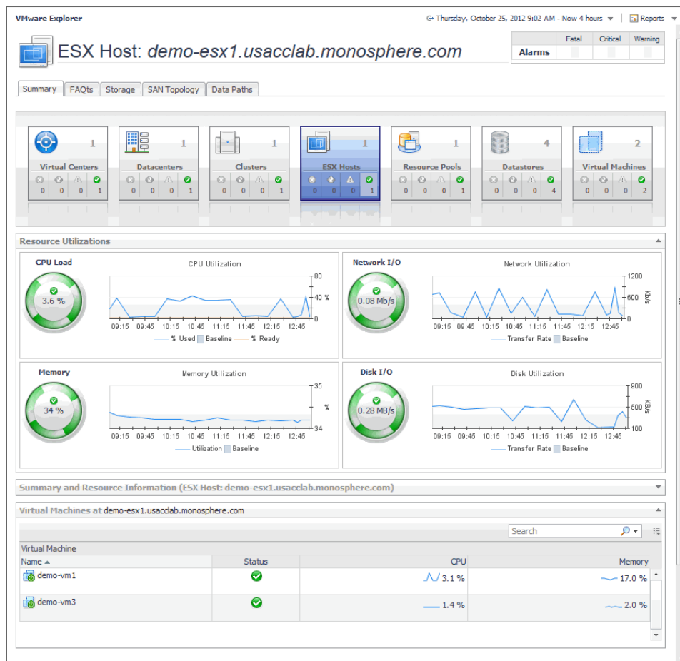
Figure 65. Summary tab
