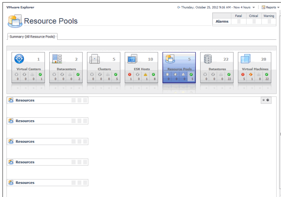
Figure 68. Summary (All Resource Pools) tab
