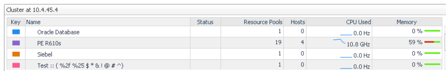
Figure 26. Cluster details
