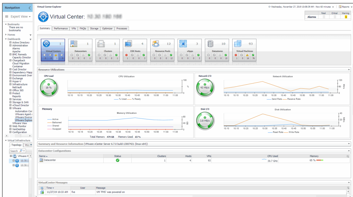
Figure 12. VMware Explorer
