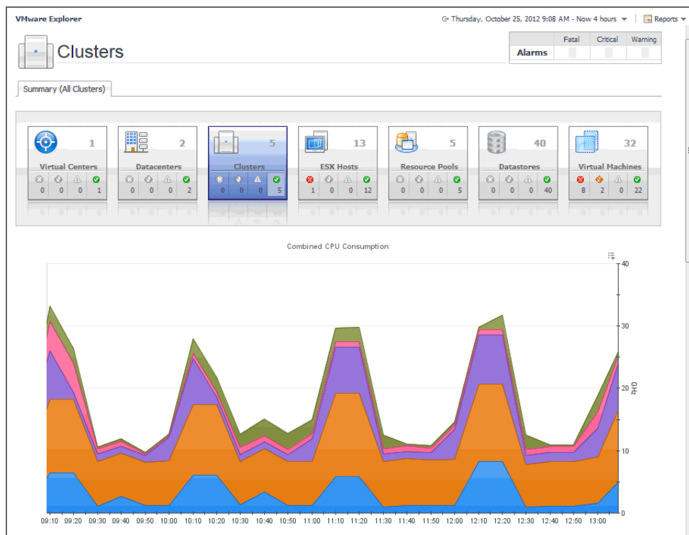
Figure 66. Summary (All Clusters) tab
