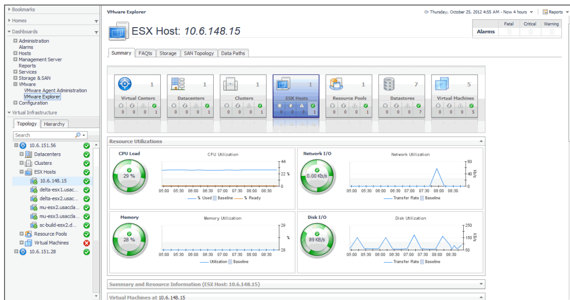
Figure 3. Foglight for VMware Browser Interface
