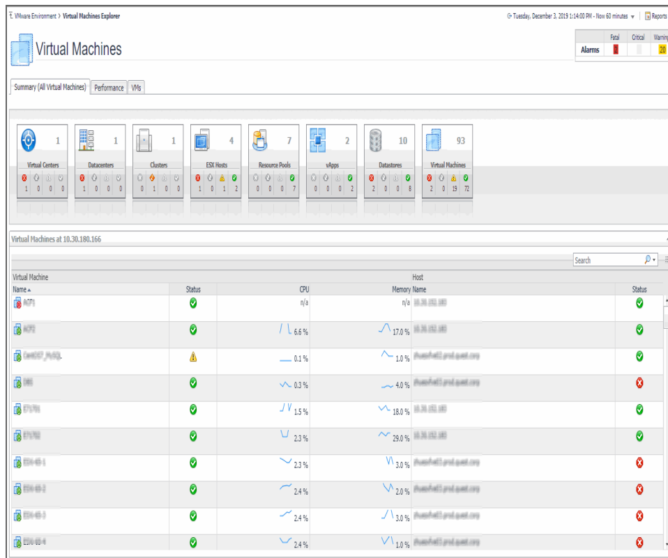
Figure 70. Summary (All Virtual Machines) tab
