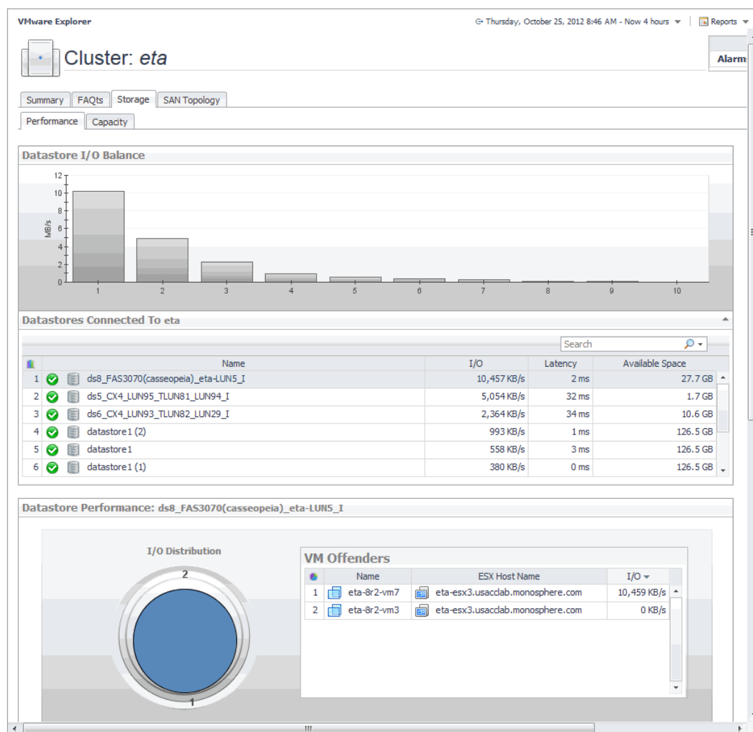
Figure 61. Storage tab (Cluster)
