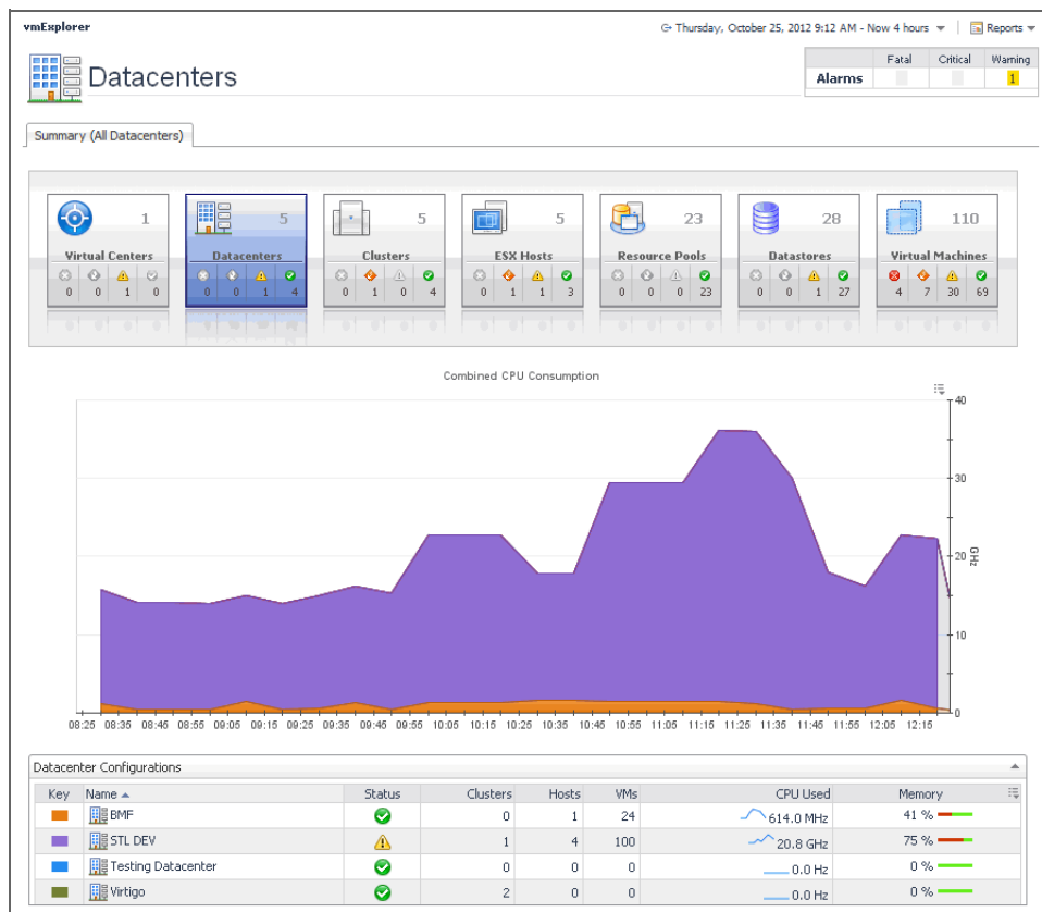
Figure 67. Summary (All Datacenters) tab
