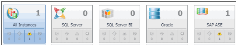
Figure 40. Database Tiles
