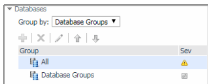
Figure 42. Database Groups
