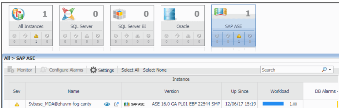
Figure 41. Database Instances
