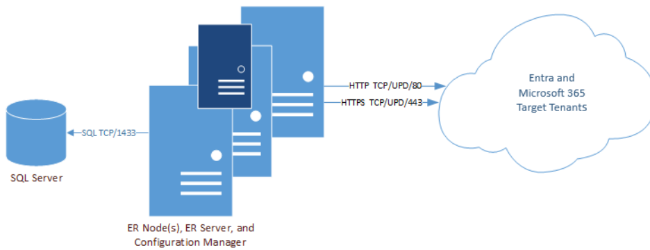
Figure 5. Ports used by Microsoft Entra ID and Microsoft 365 collections (Exchange Online, MS Teams, OneDrive, and SharePoint Online)
