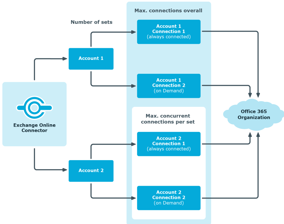
Figure 2: Determining sessions
