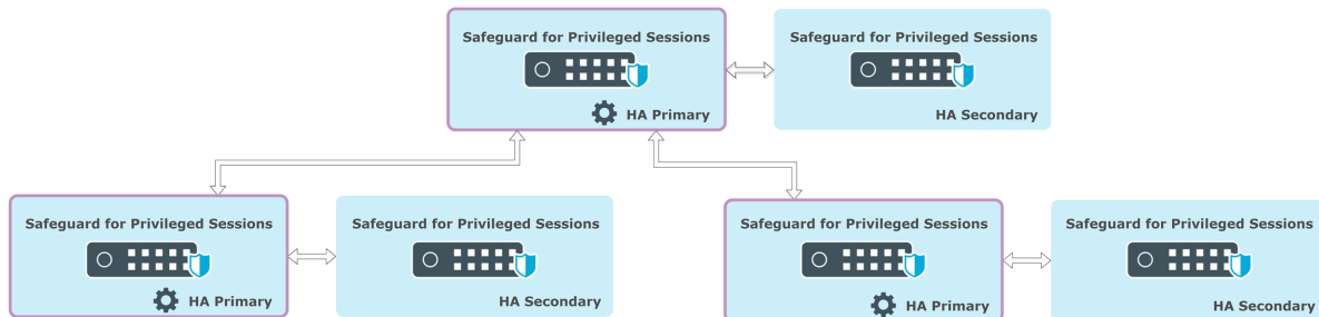
Figure 2: Clustering in SPS
