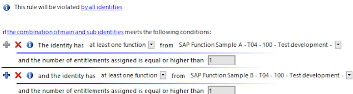
Figure 5: Condition for SAP functions
