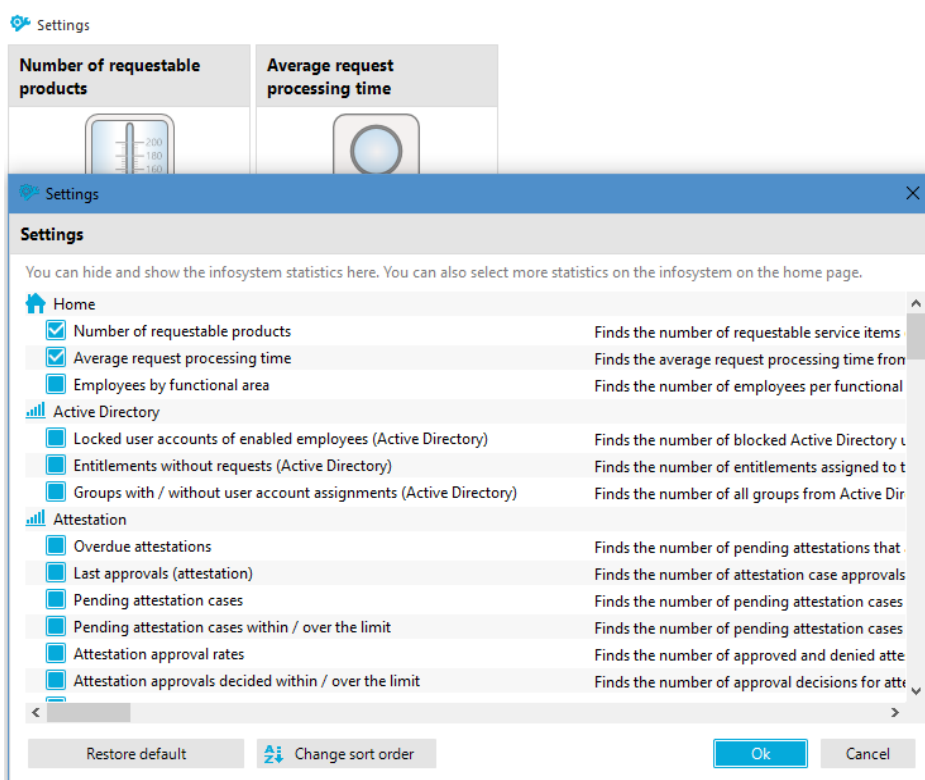
Figure 2: Statistics settings
