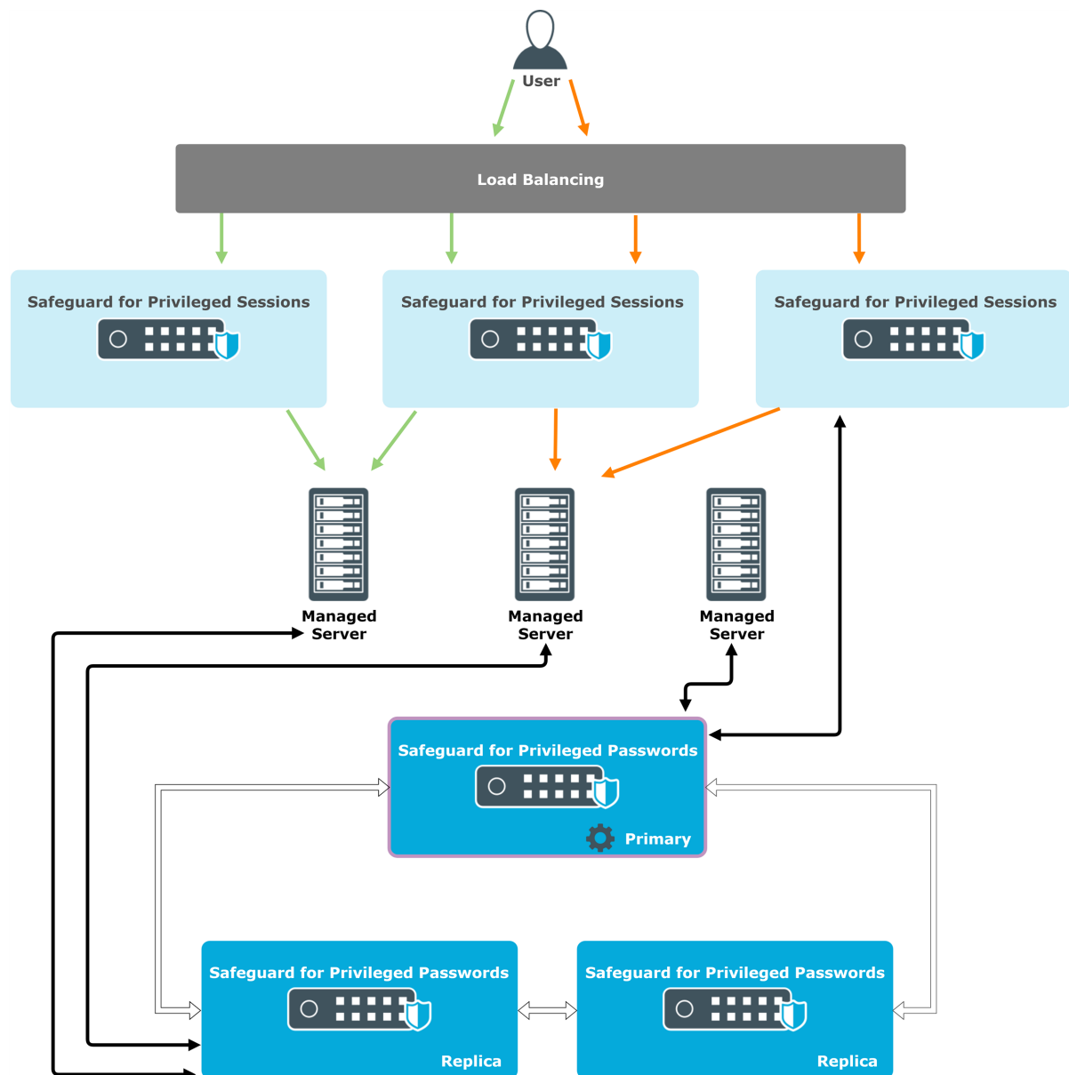
Figure 9: SPS-initiated workflow
