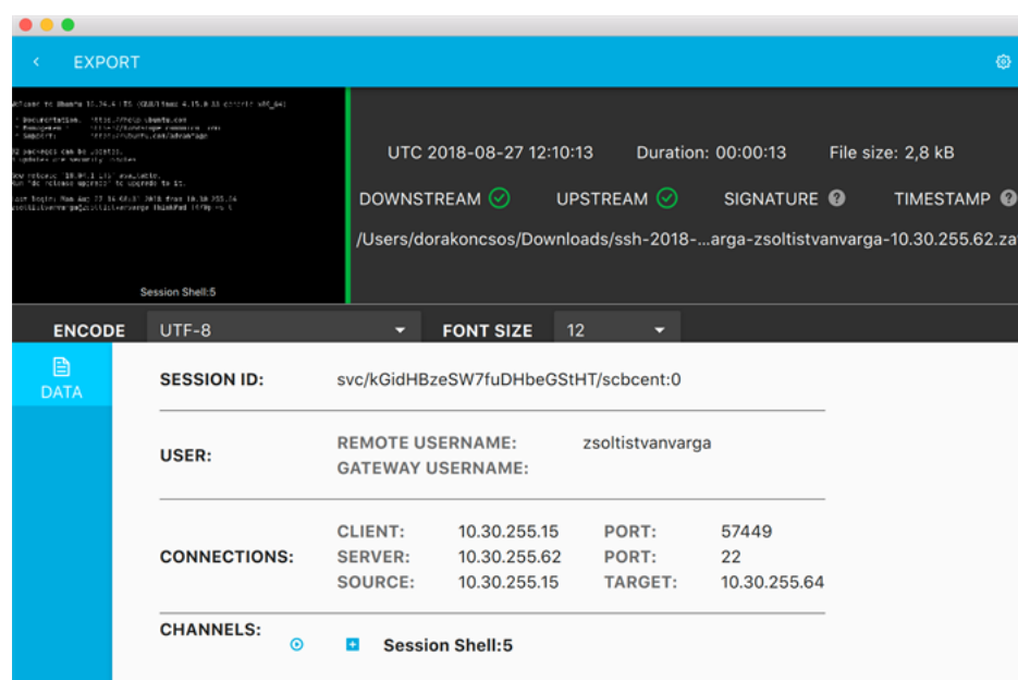
Figure 6: Replaying an audit trail
