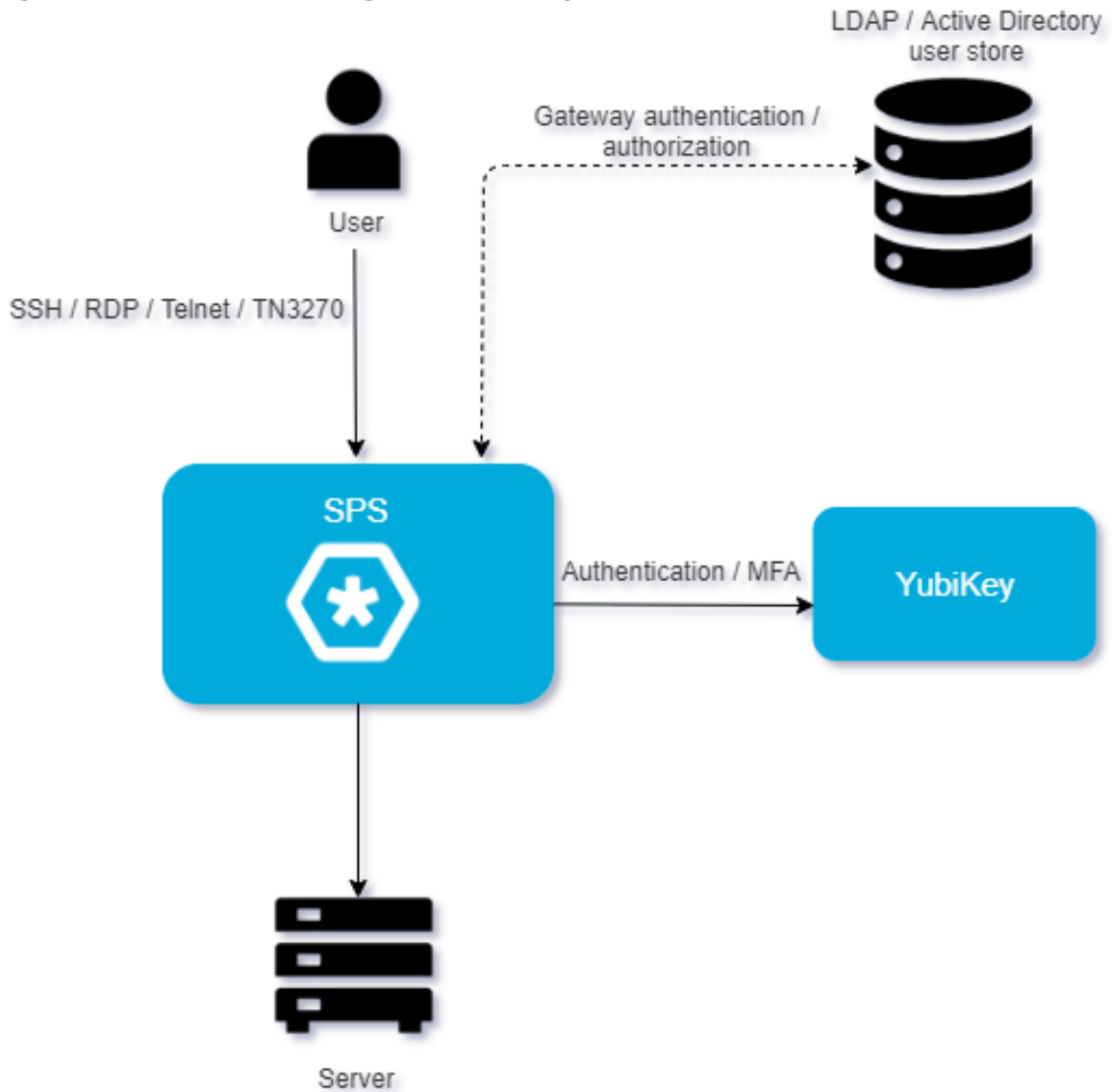
Figure 1: SPS interworking with YubiKey
