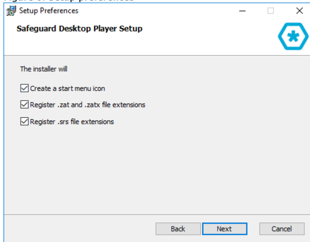
Figure 6: Setup preferences
