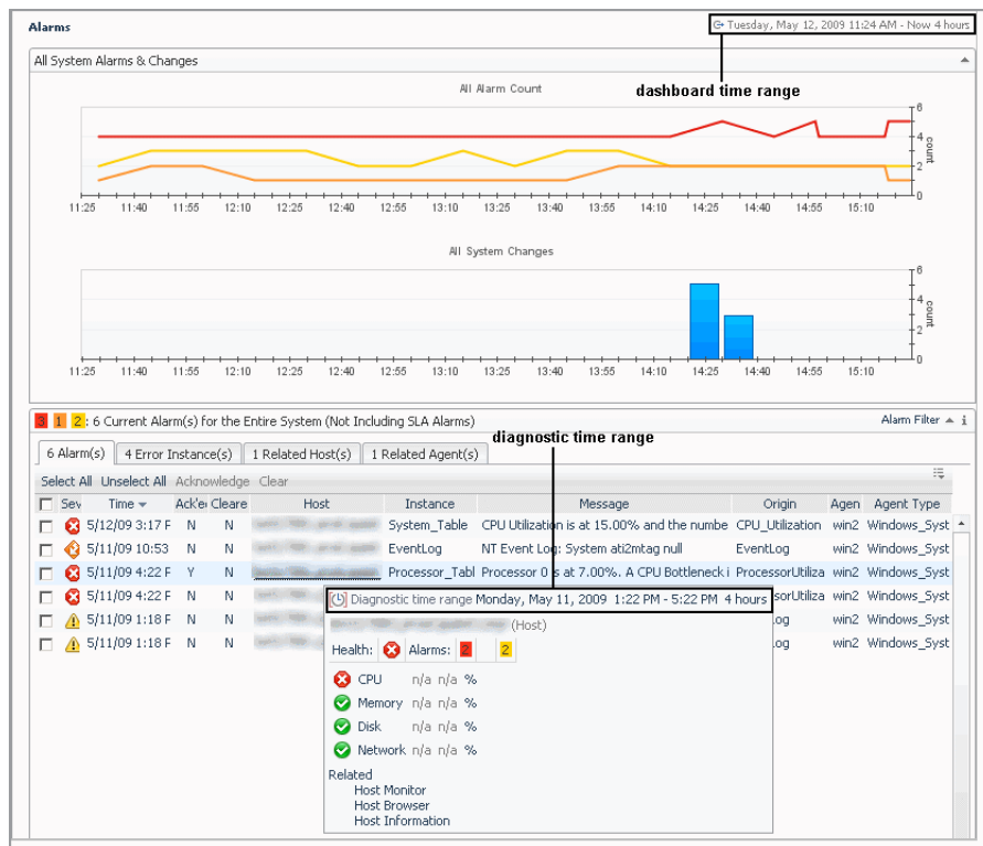
Figure 17. A diagnostic time range is displayed at the top of the summary.
