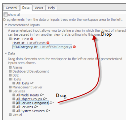
Figure 22. Drag and drop a data element.
