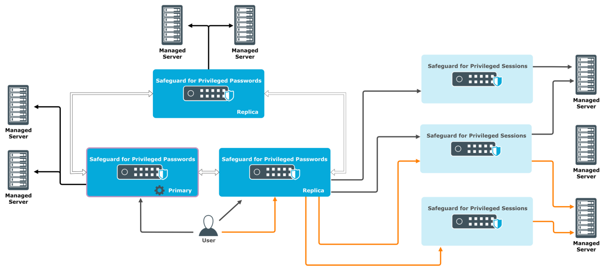
Figure 8: SPP-initiated workflow
