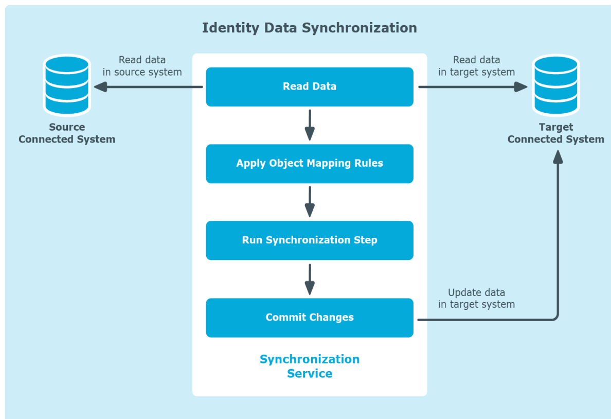
Figure 8: Identity Data Synchronization
