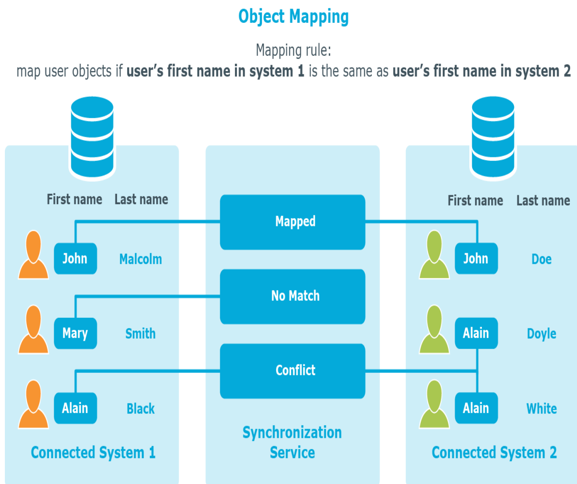
Figure 12: Object mapping
