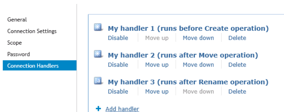
Figure 7: Connection Handlers
