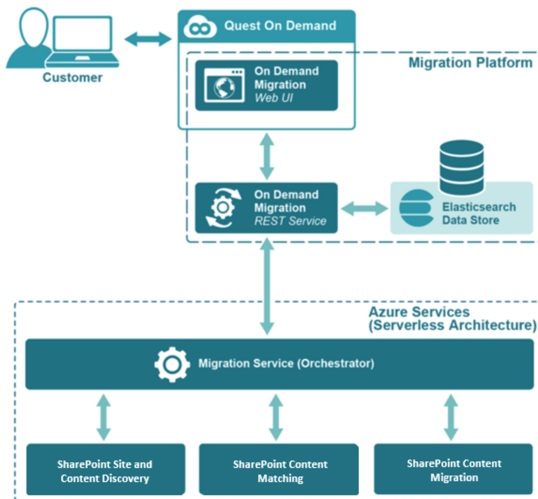
Figure 1: High-Level Architecture
