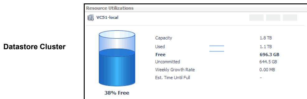
Figure 28. Datastore Cluster Resource Utilizations view
