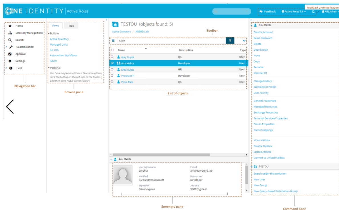
Figure 1: UI Elements
