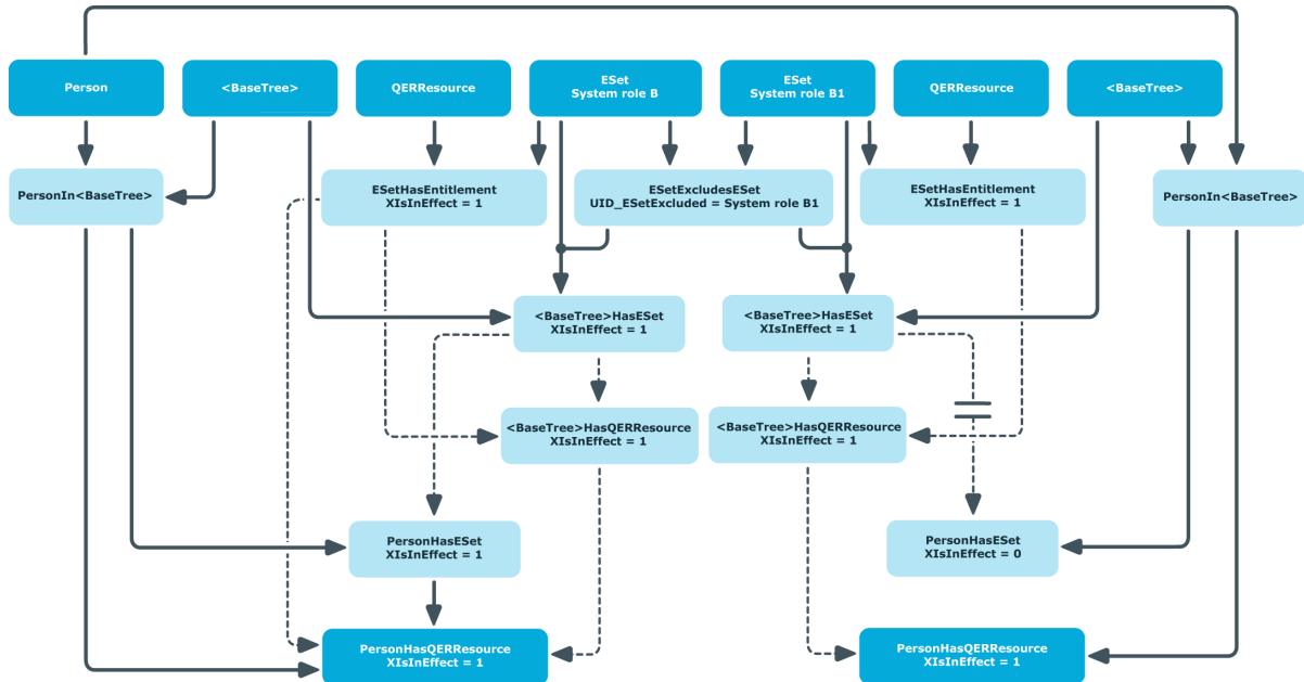
Figure 9: Inheritance by different hierarchical roles when the configuration parameter is deactivated
