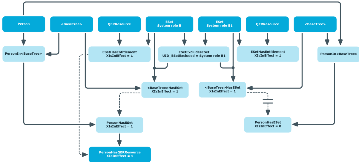
Figure 8: Inheritance by different hierarchical roles when the configuration parameter is activated
