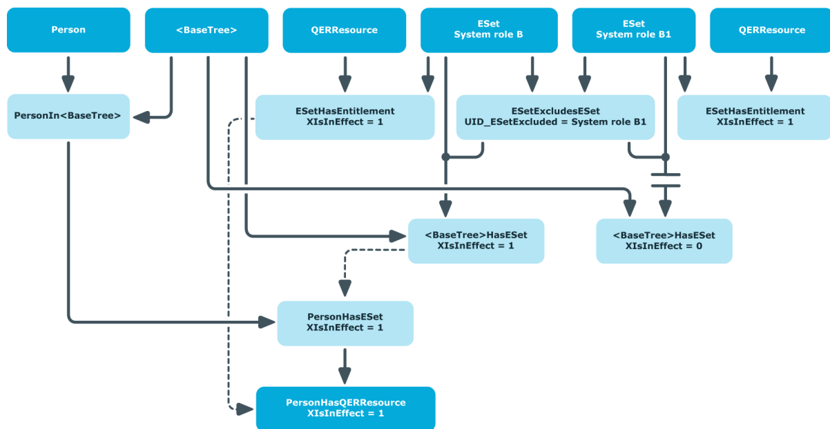
Figure 7: Inheritance by indirectly assigned system roles when the configuration parameter is activated
