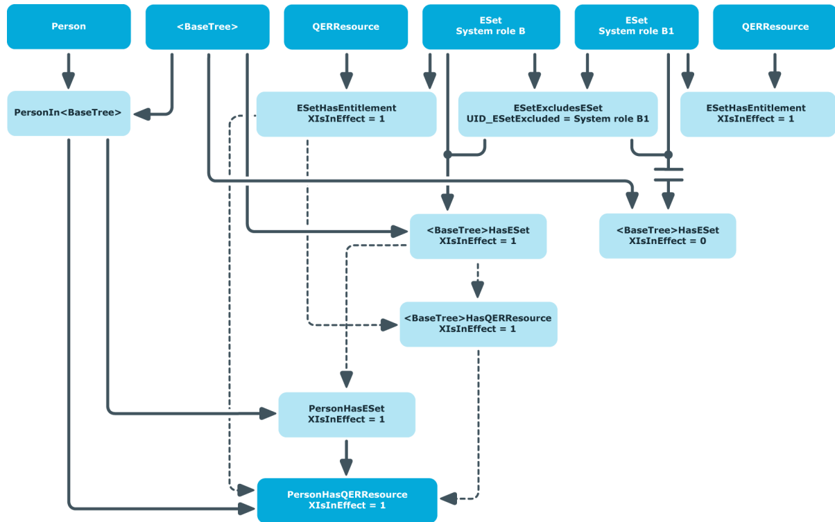
Figure 10: Inheritance through the same hierarchical role when the configuration parameter is deactivated
