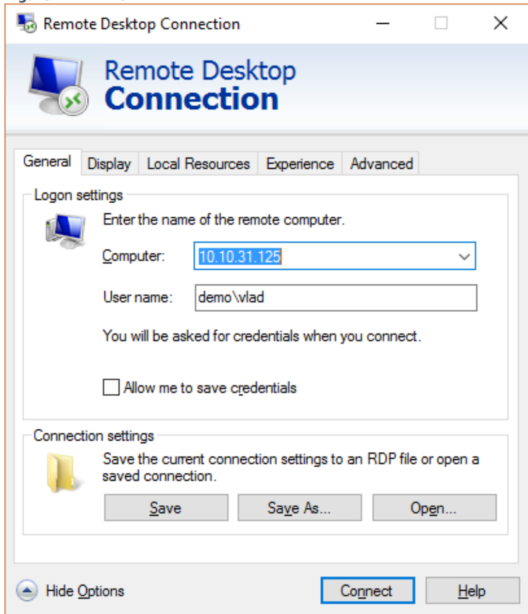
Figure 4: RDP non-NLA
