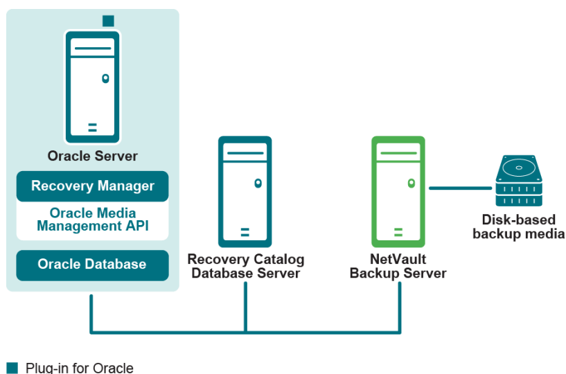
Figure 3. Single-instance non-RAC configuration
