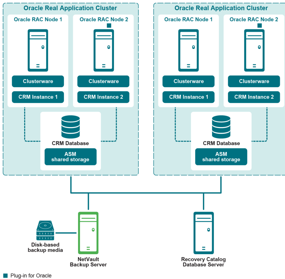
Figure 10. Multi-instance RAC to multi-instance RAC Data Guard deployment
