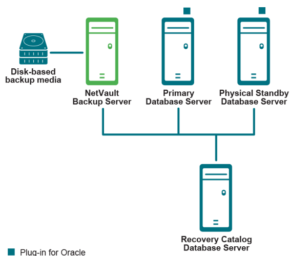
Figure 8. Single-instance to single-instance Data Guard deployment
