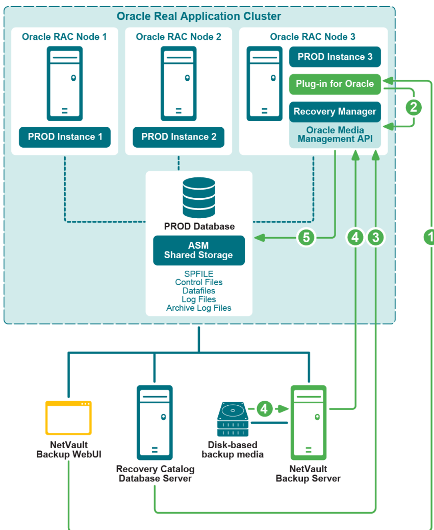
Figure 5. RMAN restore process for RAC environment
