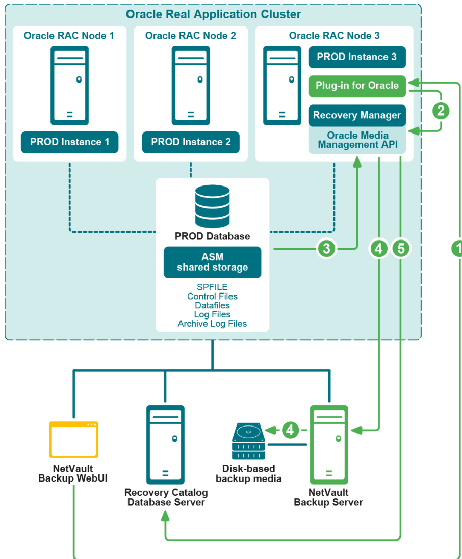
Figure 4. RMAN backup process for RAC environment
