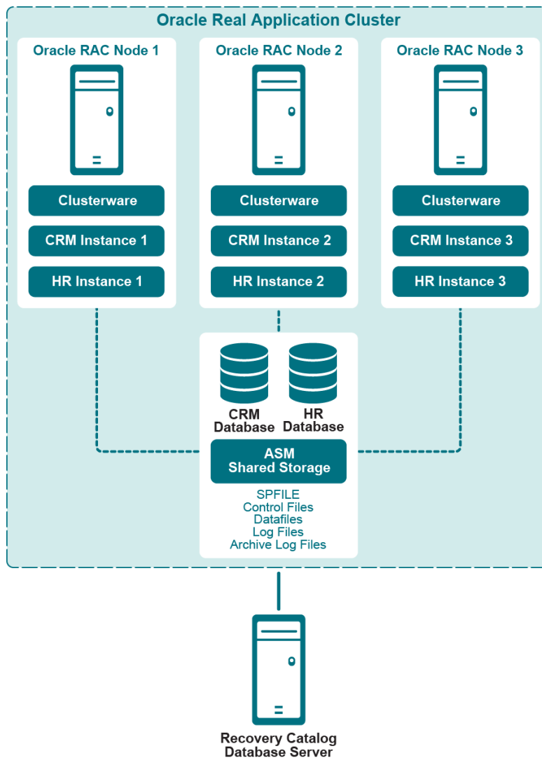
Figure 7. Supported multiple-database deployments
