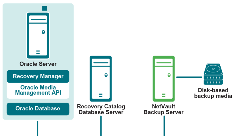
Figure 3. Single-instance non-RAC configuration
