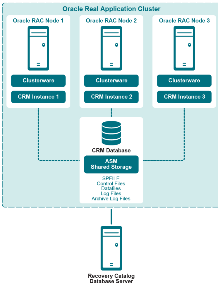
Figure 6. Supported single-database deployments
