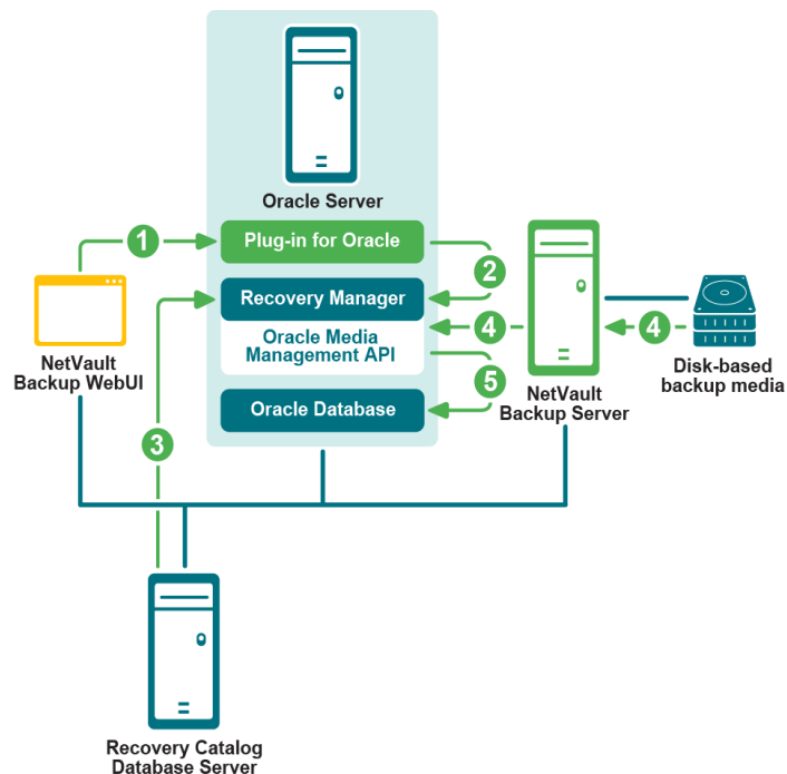
Figure 2. RMAN-based restore and recovery
