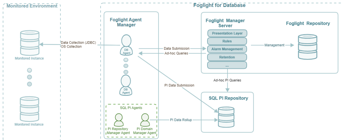
Figure 1. Foglight for Databases Components
