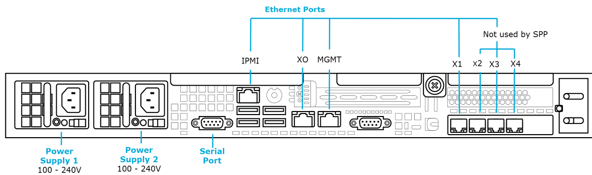
Figure 3: Back panel of 3000 Appliance
