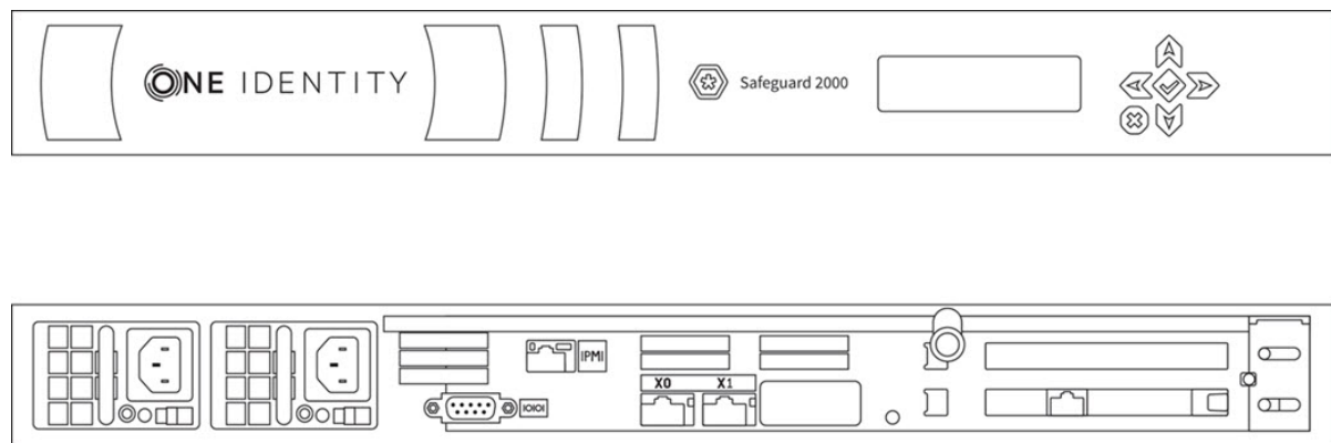
Figure 4: Front and back panel of 2000 Appliance
