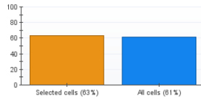
Memory Utilization
