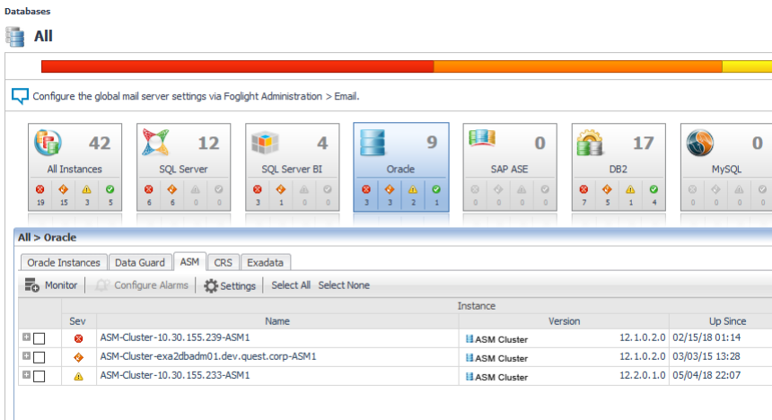
Figure 3. ASM tab
