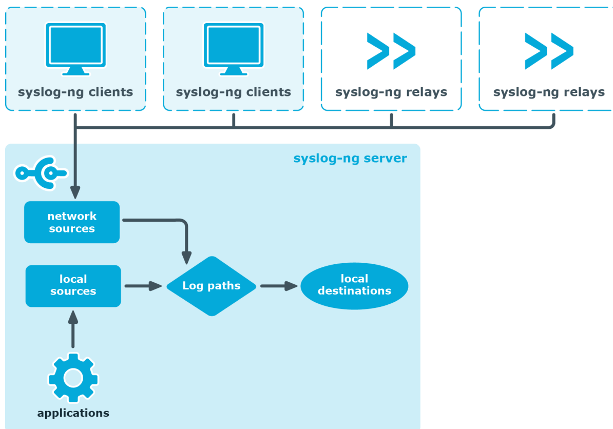
Figure 3: Server-mode operation
