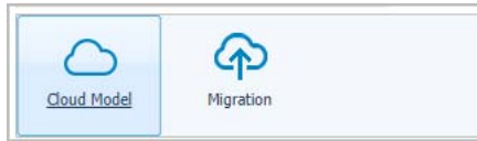
Figure 5. Menu bar
