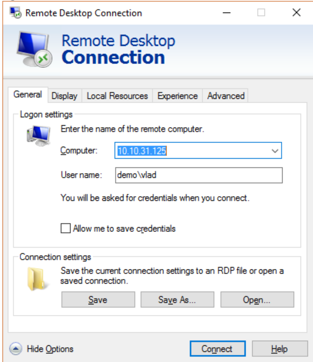
Figure 4: RDP non-NLA
