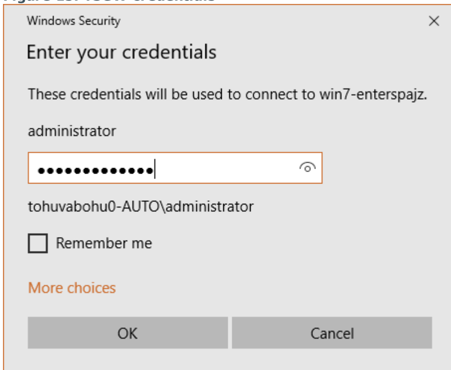
Figure 15: TSGW credentials
