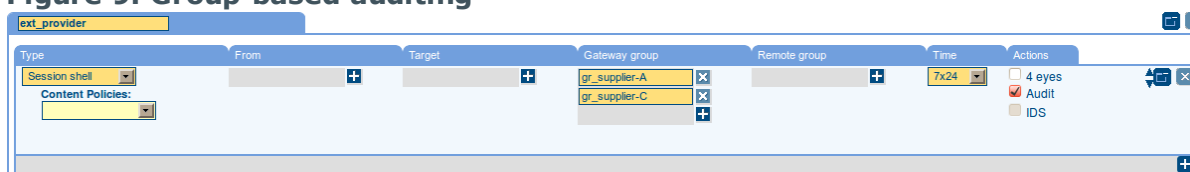
Figure 9: Group-based auditing
