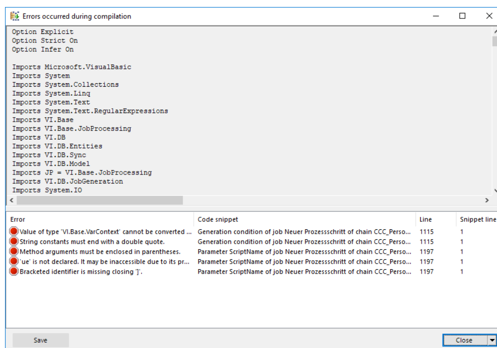
Figure 4: Error Message Log
