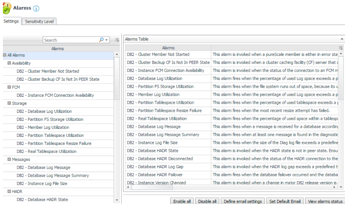
Figure 3. Use the Alarms view to edit alarm rules.
