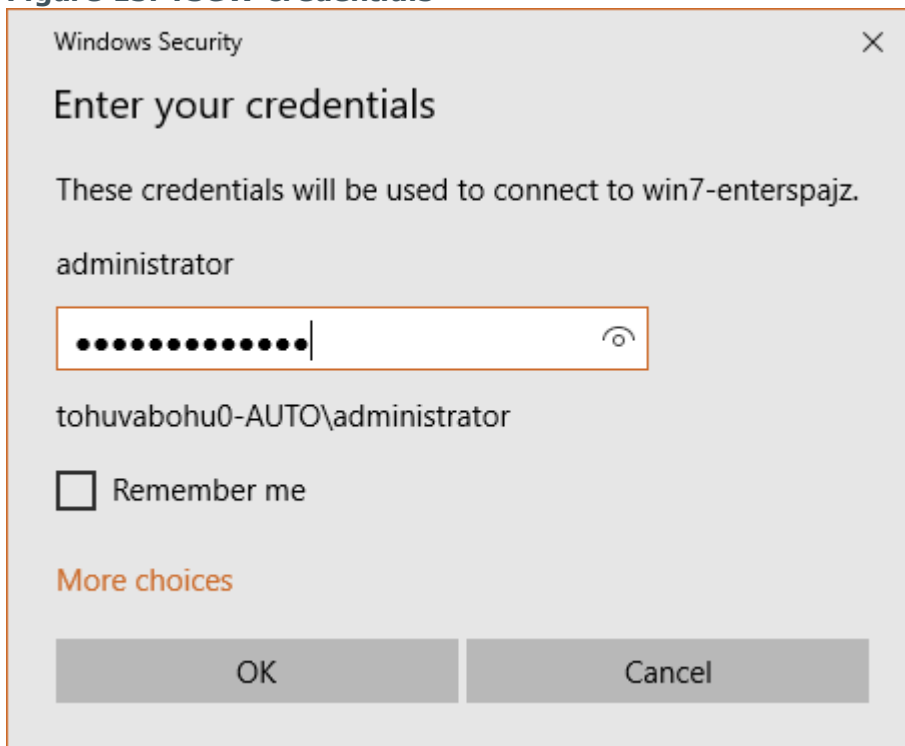
Figure 15: TSGW credentials
