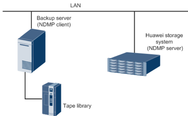
Figure 1. Three-way—remote—topology
