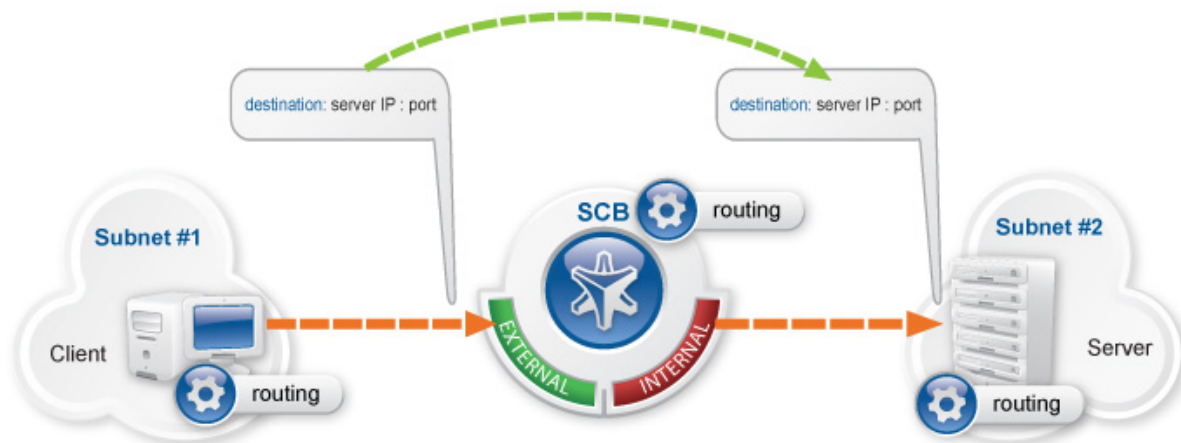
Figure 1: SPS in transparent mode
