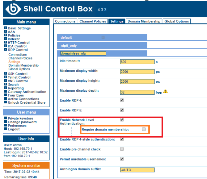
Figure 5: RDP Control > Settings — RDP settings domainless NLA
