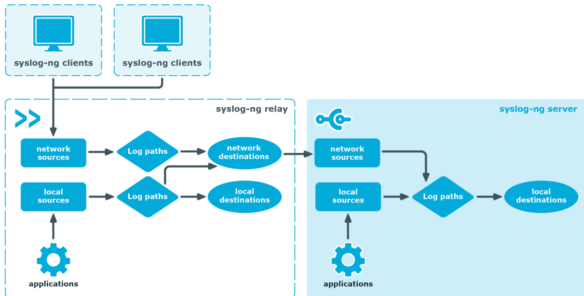
Figure 2: Relay-mode operation
