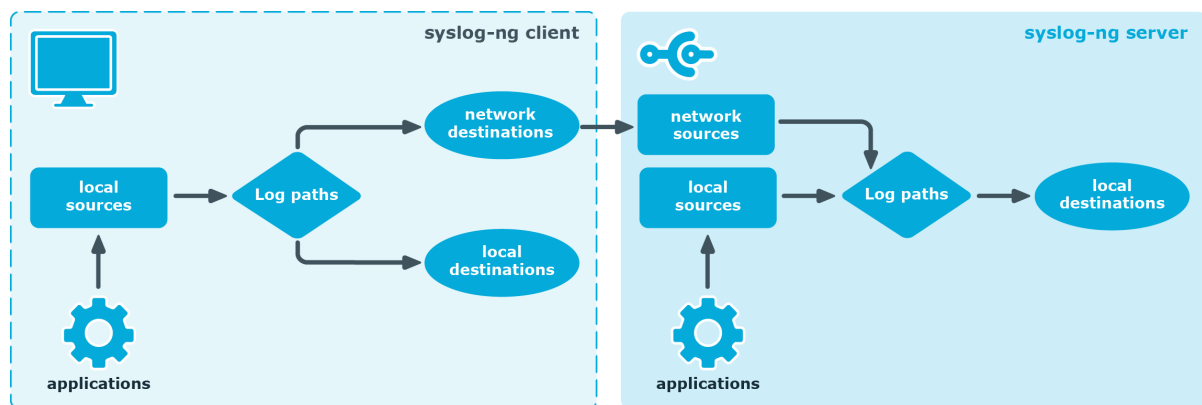
Figure 1: Client-mode operation
