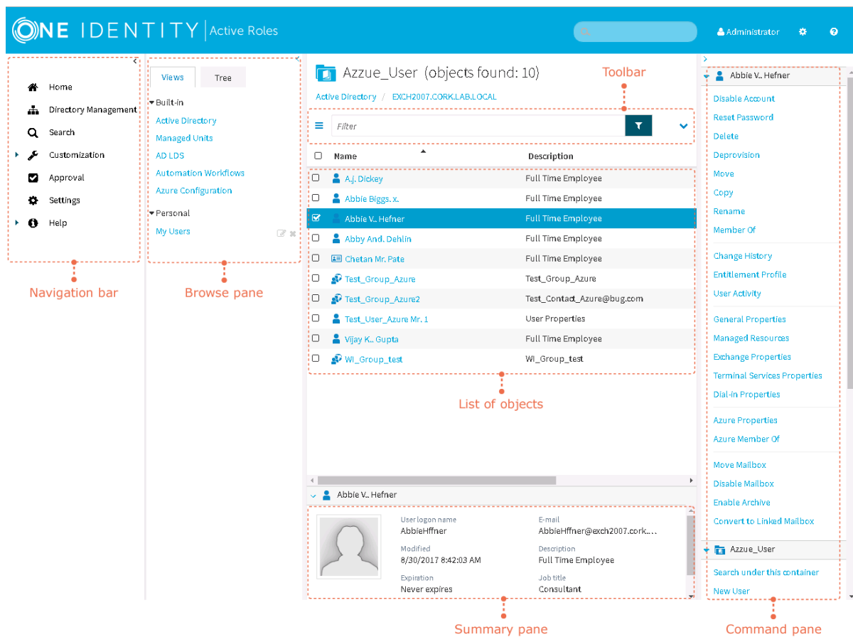
Figure 1: UI Elements
