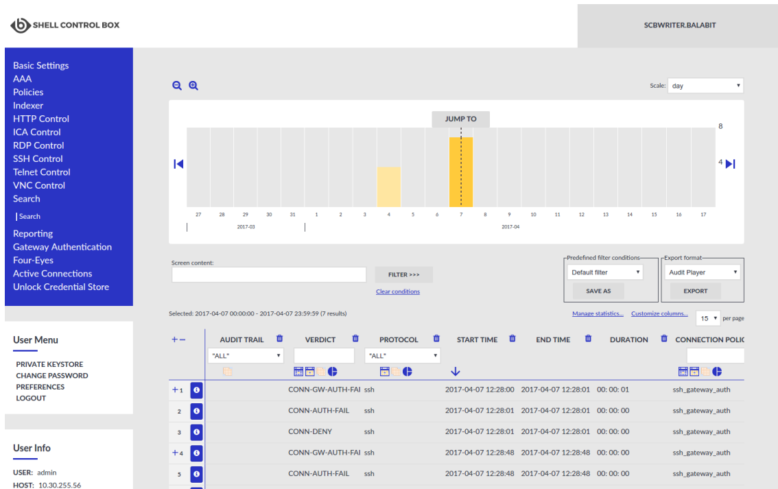
Figure 1. The Search page after the facelift
