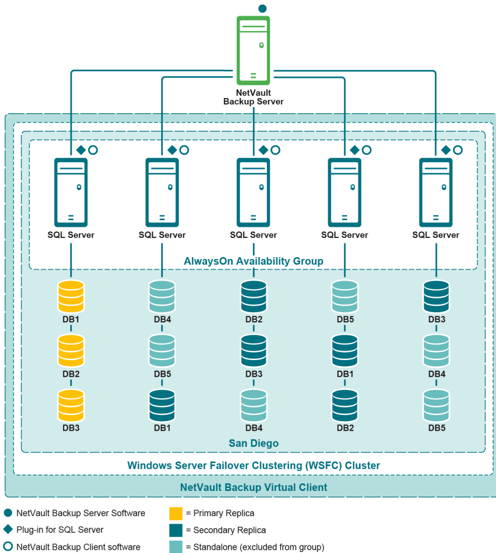
Figure 2. AlwaysOn deployment
