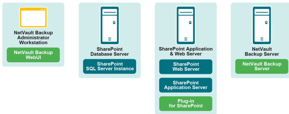
Figure 2. Plug-in deployed in a Small Farm deployment
