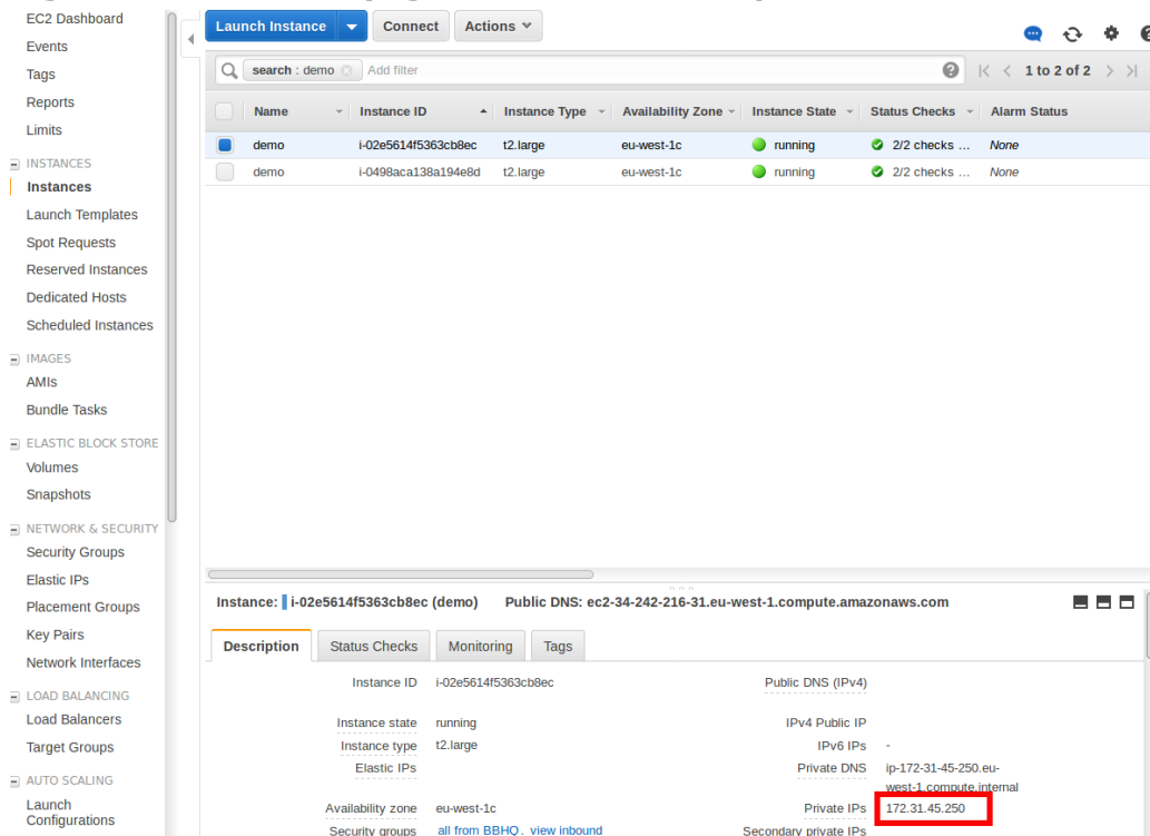
Figure 13: Instances page – Instance description
