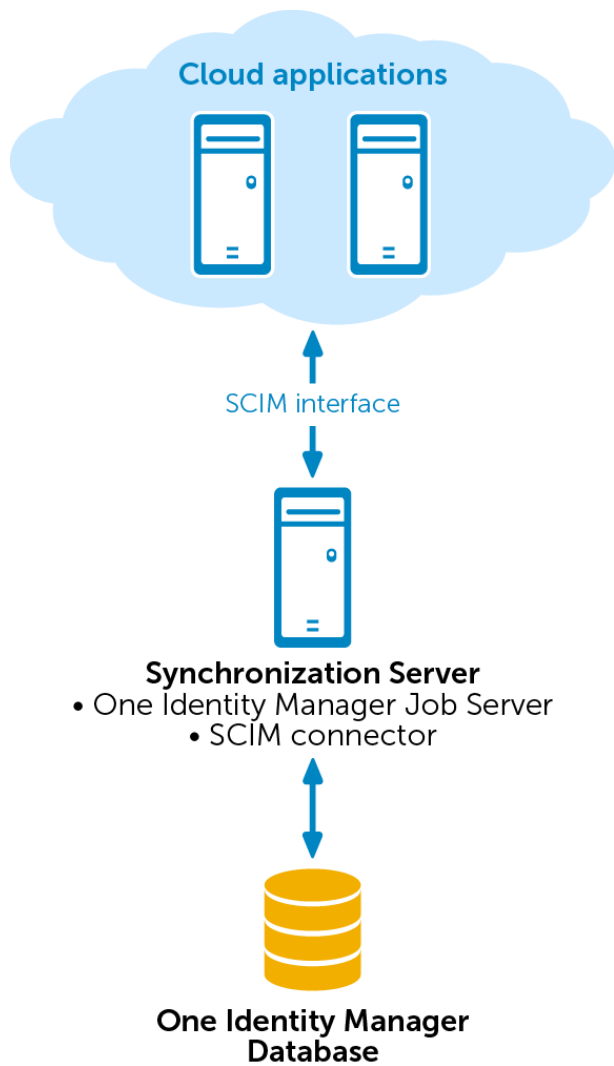
Figure 2: Synchronization topology
