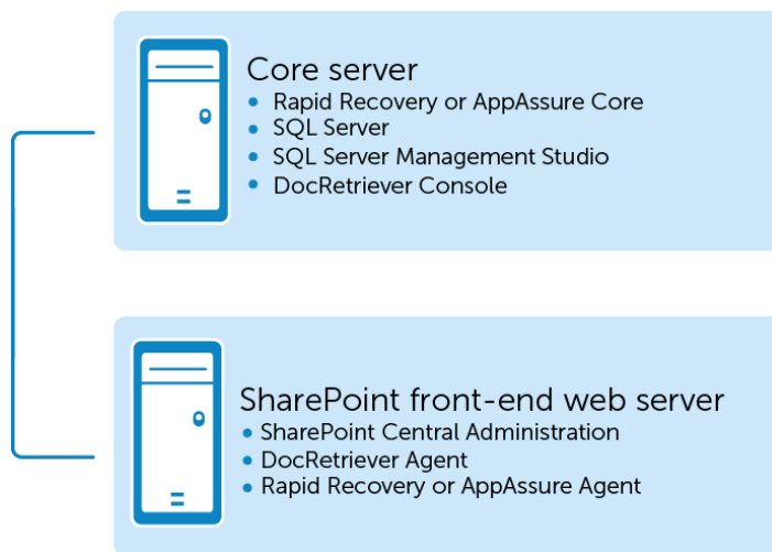
Figure 1. DocRetriever in standard mode, two servers
